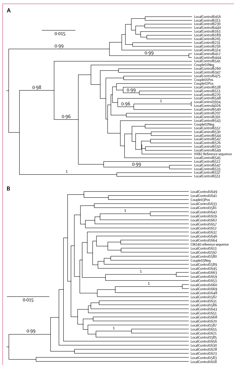
Figure: Phylogenetic trees of pol sequences
